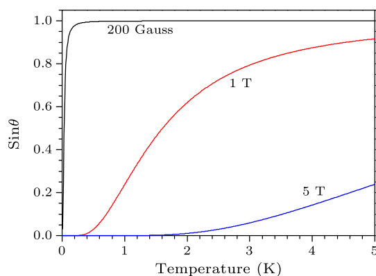
Fig. 4. Temperature dependence of the Larmor precession signal under different magnetic fields of 200 Gauss, 1 T, and 5 T.
